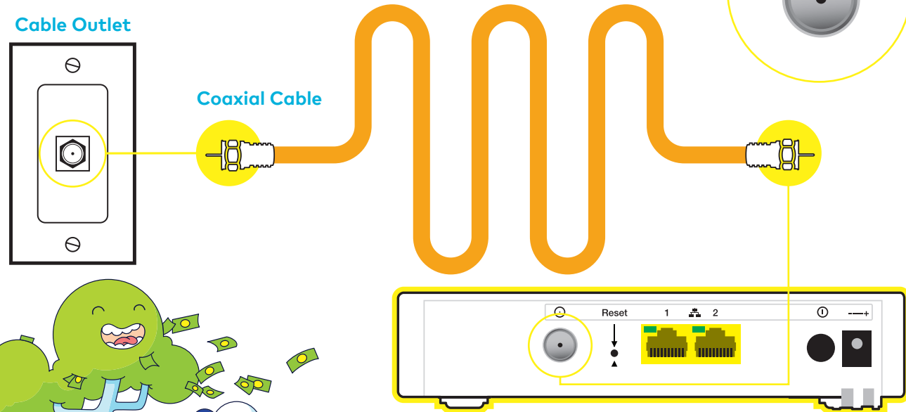
Back of Technicolor Modem
